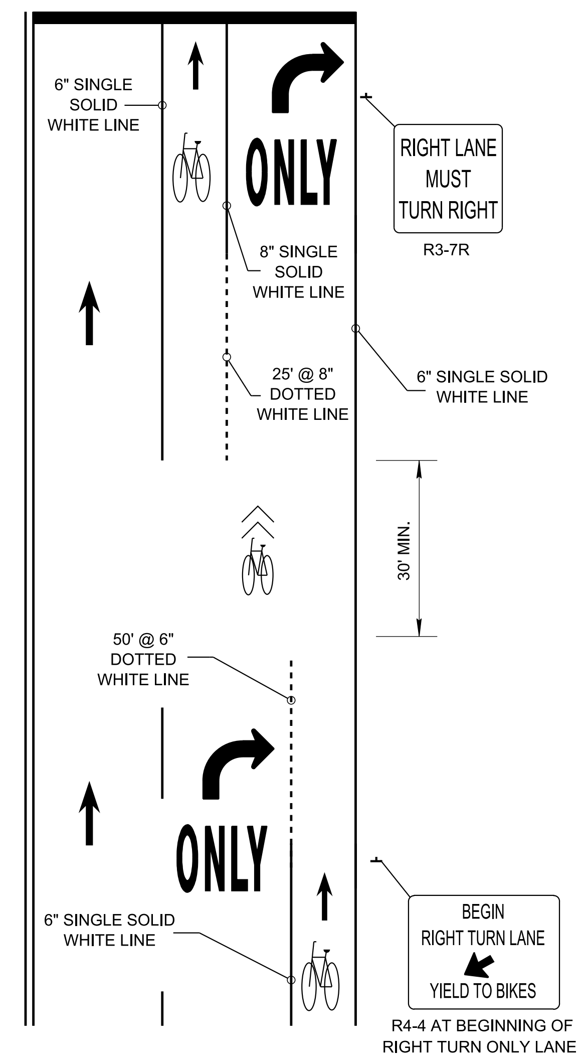
TYPICAL BICYCLE LANE TREATMENT AT A RIGHT TURN DROP LANE
