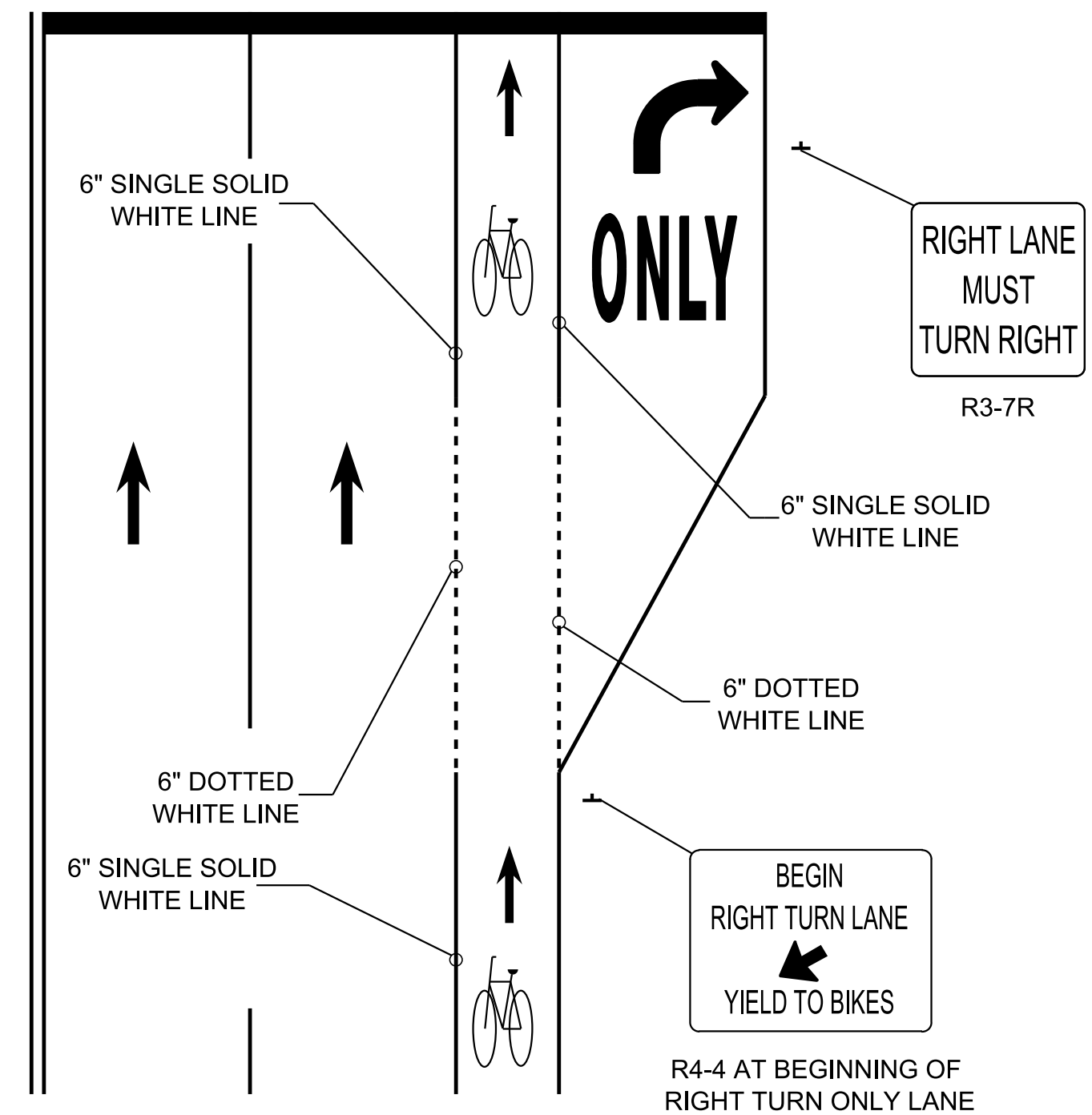
TYPICAL BICYCLE LANE TREATMENT AT A RIGHT TURN ONLY LANE
