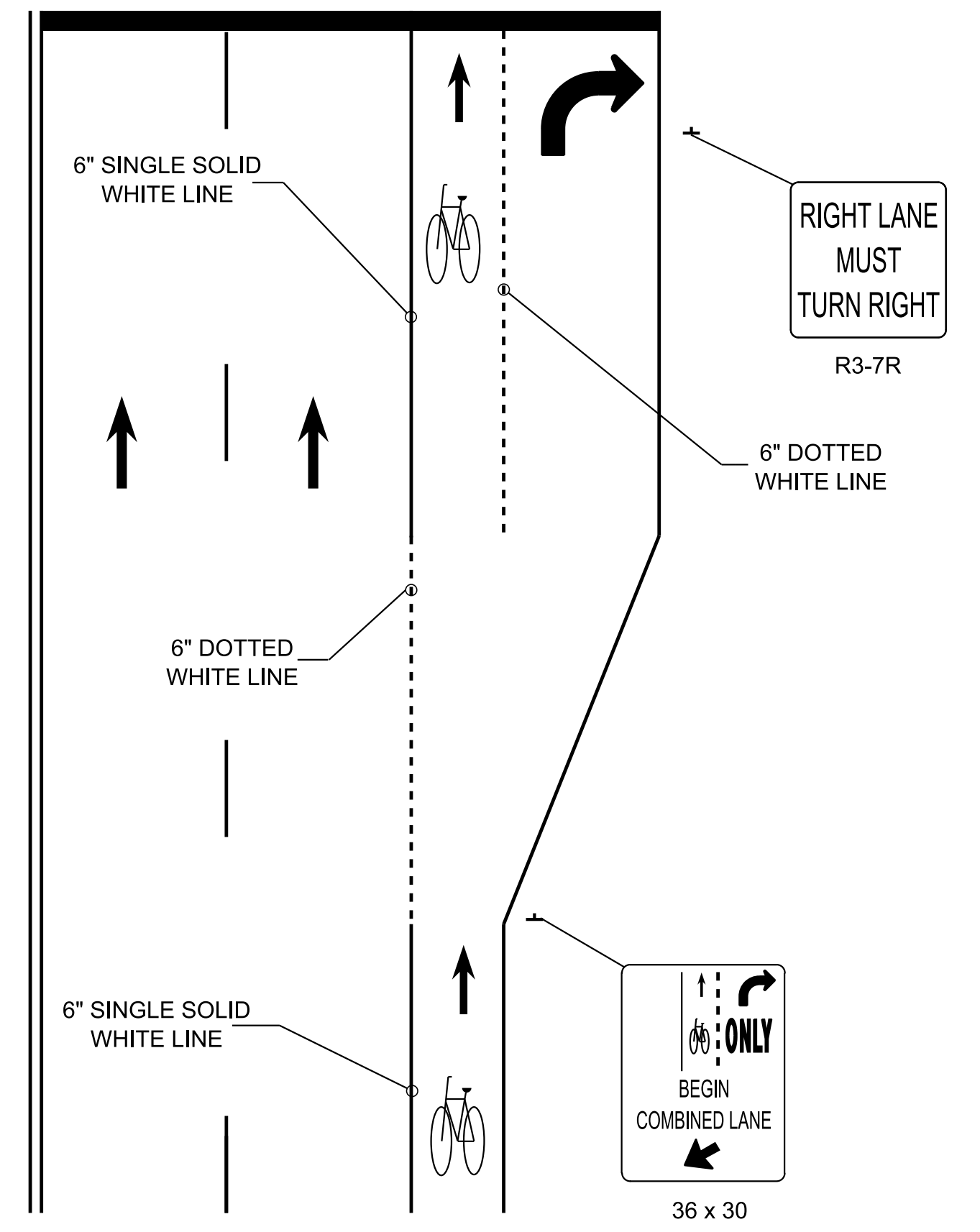
RIGHT-TURN LANE SHARED BY BICYCLISTS AND MOTORISTS (TO BE USED WITH LIMITED ROW ON SLOW SPEED ROADWAYS)
