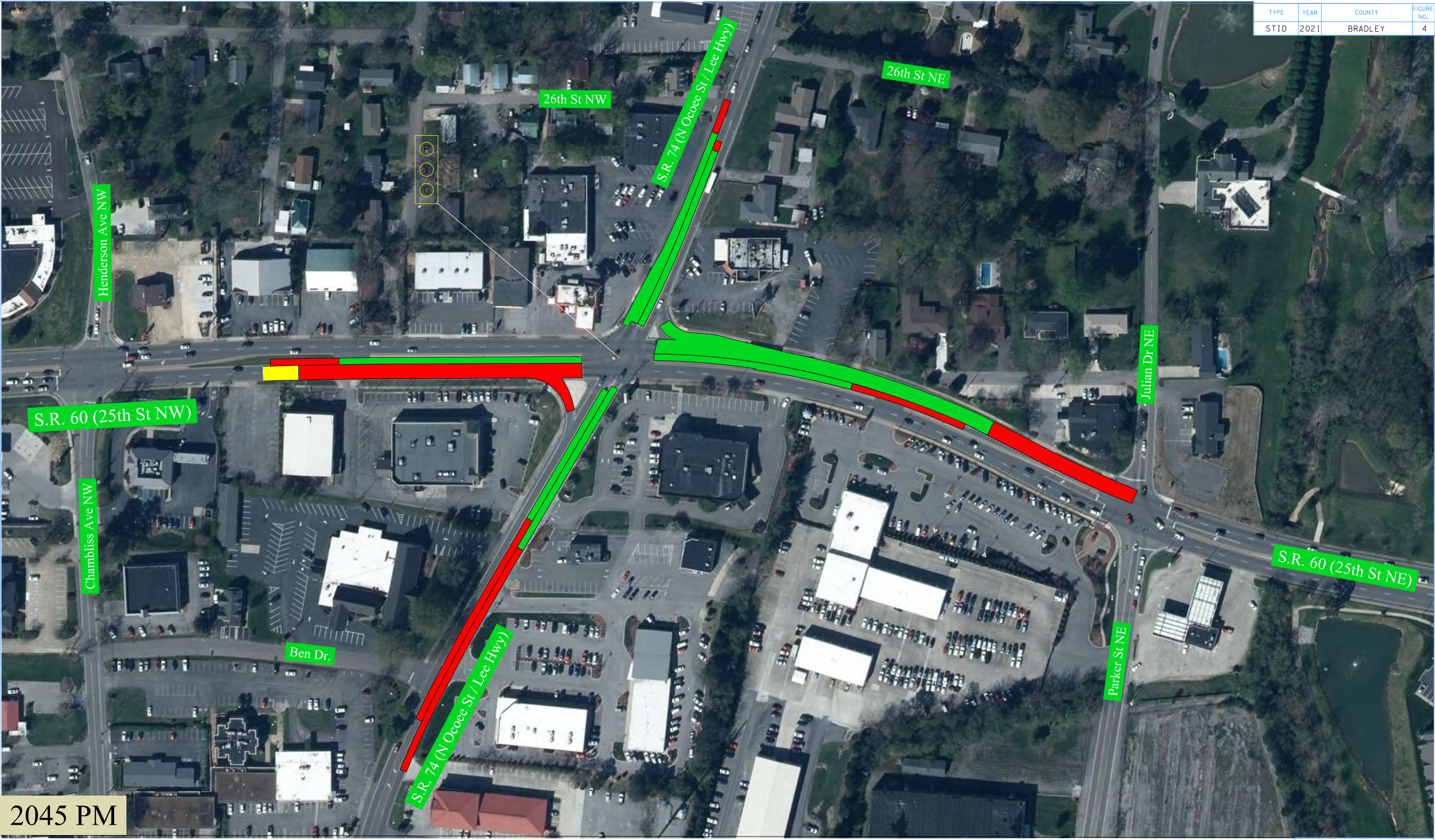
FIGURE 4 S.R. 74/S.R. 60 INTERSECTION BRADLEY COUNTY
